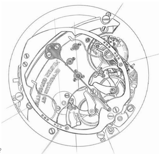
Construction drawing Hamatic
